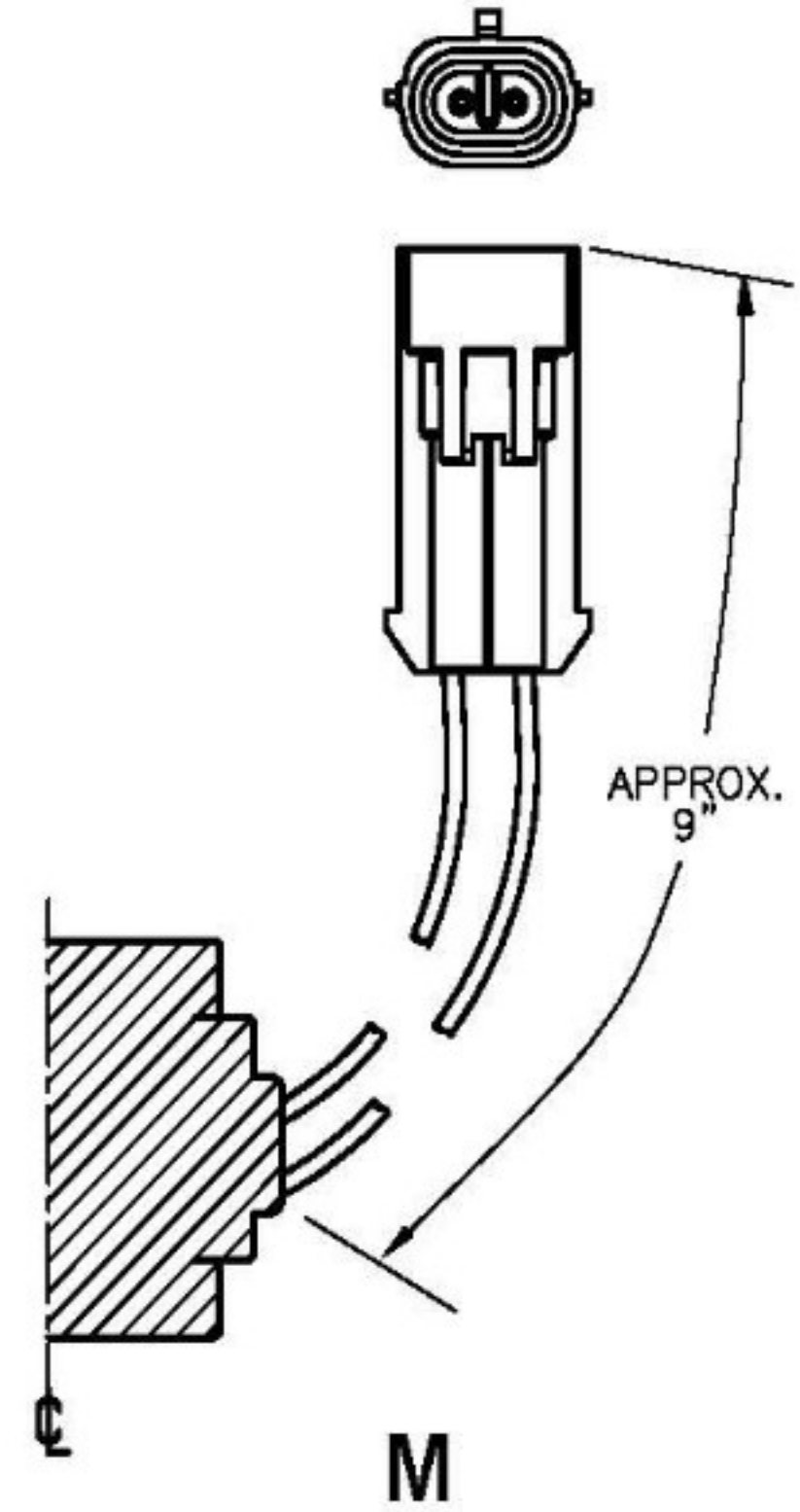
Metri-Pack® 150 Connector Mating Connector Delphi - 12052641
