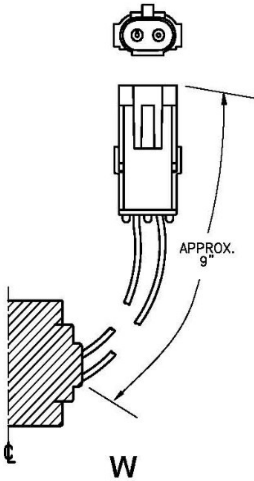
Weather-Pack® Connector Mating Connector Delphi - 12015792
